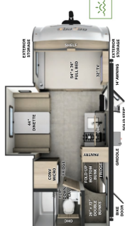
NEW! G20BH LENGTH: 21' 2" WIDTH: 7' 8" HEIGHT: 10' 4" HITCH: 480 AXL: 3288 UWV: 3906 CCC: 1092 31 GAL 27 GAL 27 GAL
