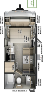
G19FD LENGTH: 20' 2" WIDTH: 7' 8" HEIGHT: 10' 1" HITCH: 432 AXL: 2947 UWV: 3417 CCC: 1016 31 GAL 27 GAL 27 GAL
