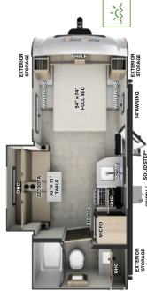
G20FBS LENGTH: 21' 2" WIDTH: 7' 8" HEIGHT: 10' 1" HITCH: 398 AXL: 3109 UWV: 3545 CCC: 853 31 GAL 27 GAL 27 GAL
