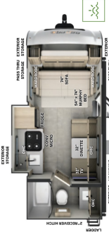
G19FBS LENGTH: 20' 2" WIDTH: 7' 8" HEIGHT: 10' 1" HITCH: 437 AXL: 3068 UWV: 3543 CCC: 894 31 GAL 27 GAL 27 GAL
