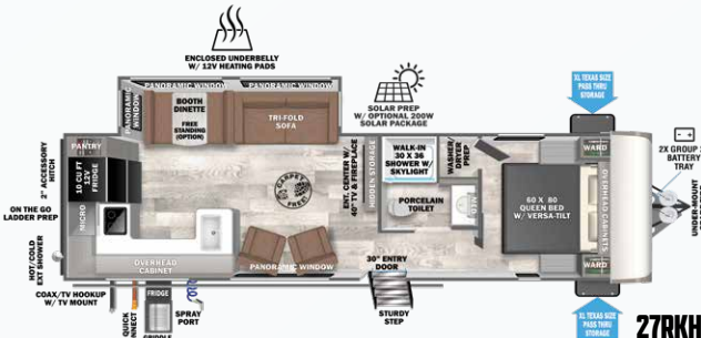
27RKHLL UVW = 6,758 lb Length = 34' 0"
