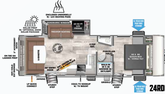
24RDHL UVW = 6,228 lb Length = 29' 11"
