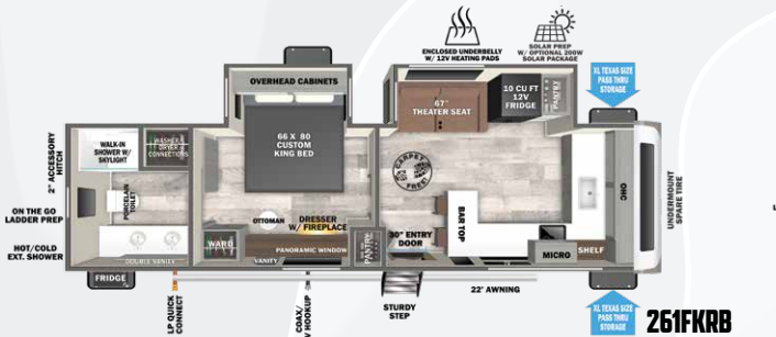
261FKRB UVW = 7,553 lb Length = 31' 5"
