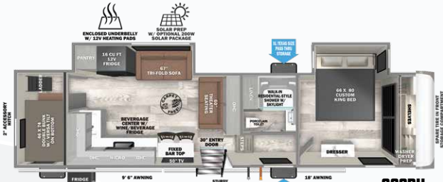
328BH UVW = 10,064 lb Length = 37' 10"
