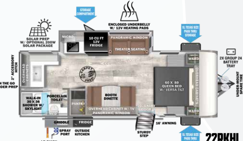
22RKHLL UVW = 6,128 lb Length = 26' 10"
