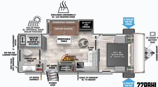
22RBHL UVW = 6,198 lb Length = 27' 6"
