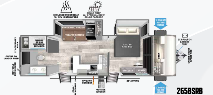
265BSRB UVW = 7,858 lb Length = 33' 2"
