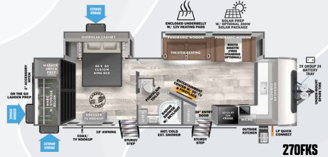
270FKS UVW = 8,243 lb Length = 33' 1"
