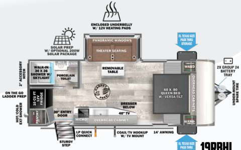
19RBHL UVW = 5,403 lb Length = 24'
