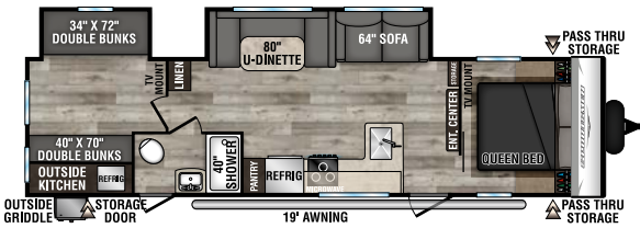
312BHKSE UVV-7,110 | Exterior Length - 35'9" | Sleeps - 10
