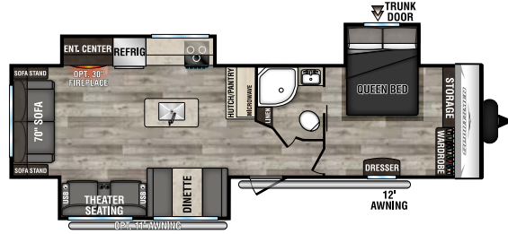
303QBSE UVV-7,550 | Exterior Length - 34'7" | Sleeps - 5
