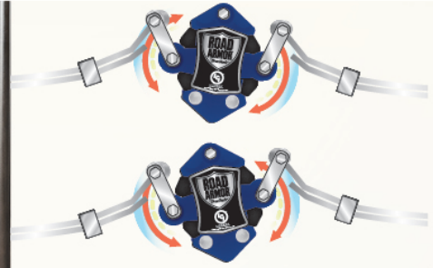
Road Armor™ Suspension w/ 360° Vibration Control Equalizes axle load to dampen shock and vibration. (TrailAir on 380/381TH models.)
