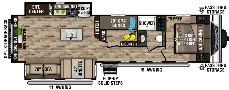
ST327VIK | 8,270 UVW | 36' 4" LENGTH | SLEEPS 11
