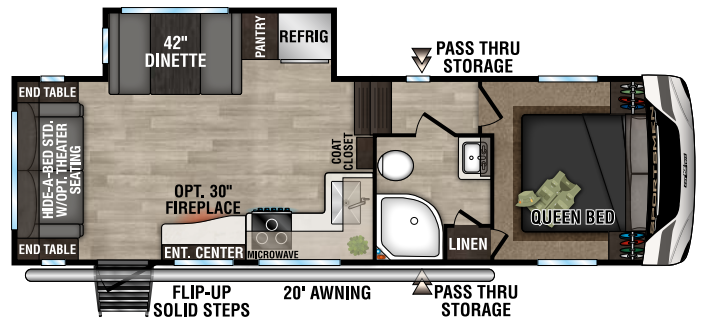
251RL UVW - 7,170 | Exterior Length - 29'4" | Sleeps - 5
