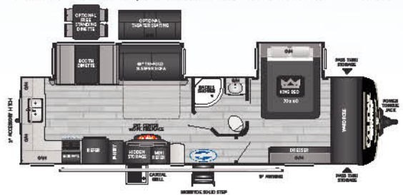
30RKDWE | Rear kitchen, king bed slide w/ large front closet
