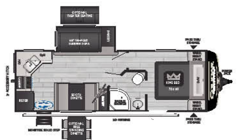
24SABWE | Dual entry rear kitchen with slide
