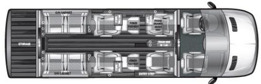
V-Drive 10OB 10 Passenger Opposing Rear Bench Seats Full or Arched Wall
