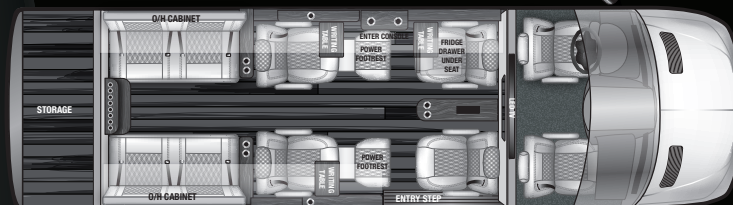
V-DRIVE 10OB 10OB/OBR Opposing Bench Seating, Full Front Wall Partition
