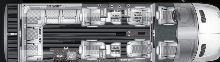
V-DRIVE 10RJ 10RJ/10RJA J Lounge Seating, Full Front Wall Partition
