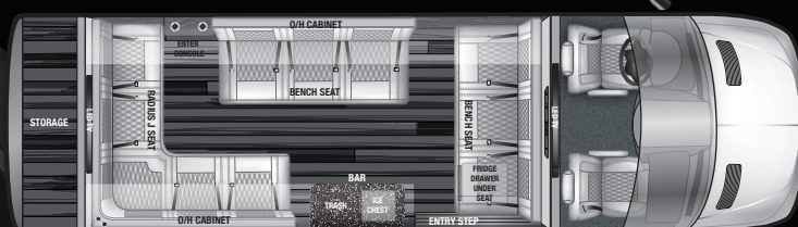
12LI/12LIA Rear J Lounge Seating, Full Front Wall Partition
