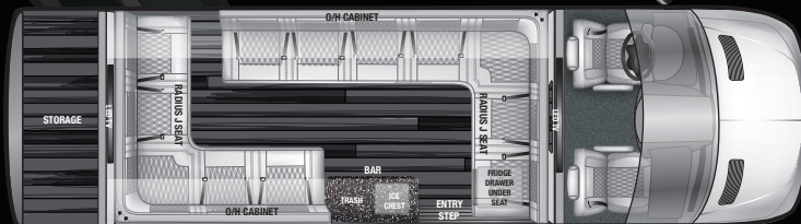
12LJ/12LJA J Lounge Seating, Full Front Wall Partition
