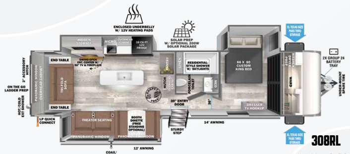
308RL UVW = 9,688 lb Length = 37' 11"
