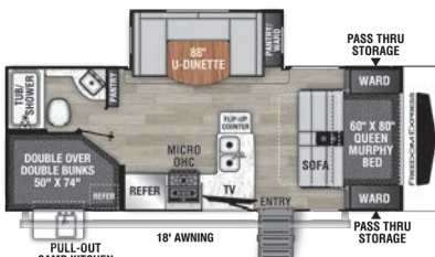
238 BHS / Exterior Length 25' 9"
