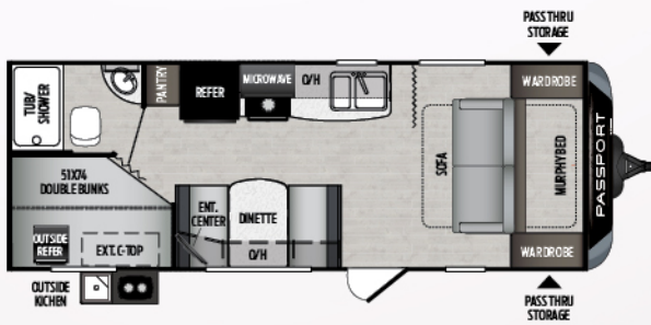
239ML | Murphy bed, bunkhouse Weight: 4140 LBS. | Length: 25' 5"
