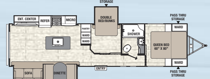
323 BHDSLE / Exterior Length 36' 11"
