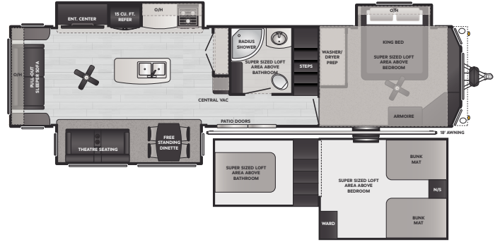
39/391FLFT | WEIGHT 12907 | LENGTH 40' 11"
