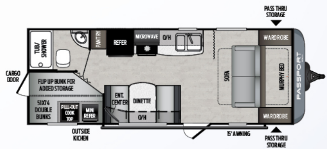
239MLWE | Murphy bed, bunkhouse with outside kitchen Weight: 4402 lbs | Length: 25' 5"
