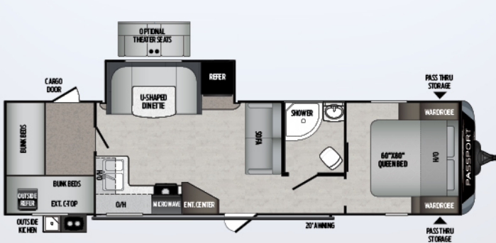
3100QB | Quad bunk w/ outside kitchen Weight: 6405 lbs | Length: 35' 11"
