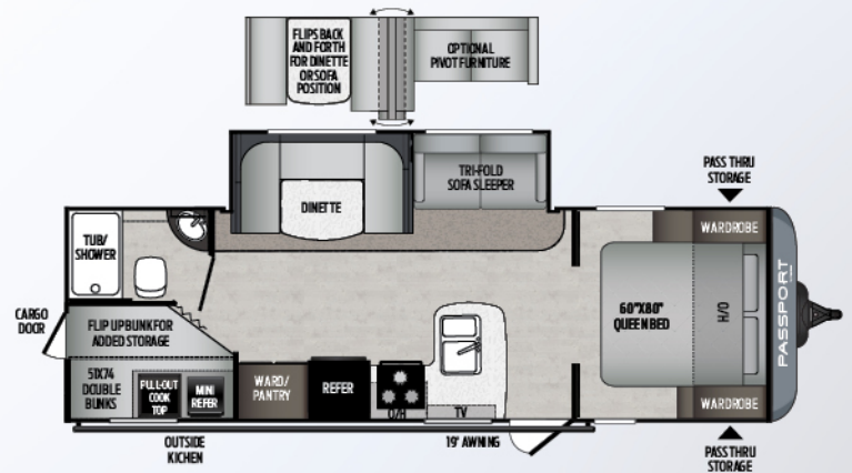
267BHWE | Super slide, bunkhouse w/ 60" x 80" queen bed Weight: 5550 lbs | Length: 30' 6"
