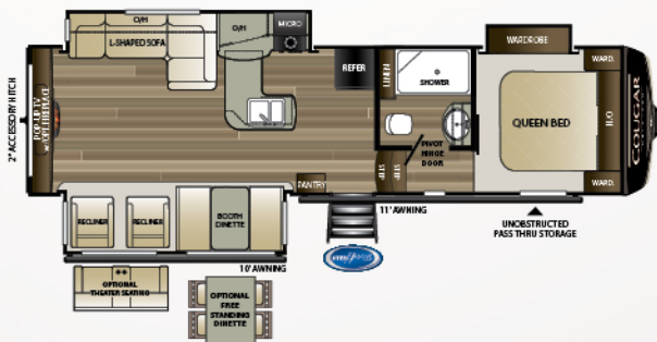
29RES | Rear entertainment, three slides Weight: 8780 LBS. | Length: 32'10"
