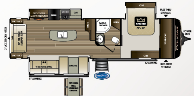
32RLI | Rear living room, three slides w/ bedroom slide Weight: 8416 LBS. | Length: 35' 11"
