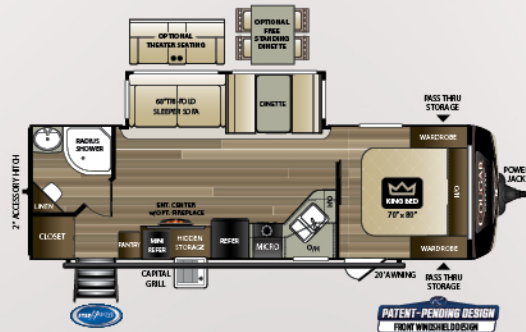
26RBS | Rear bath, slide and outside kitchen Weight: 6604 LBS. | Length: 29' 11"
