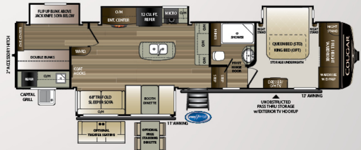
369BHS | Bunkhouse, large outside kitchen Weight: 11547 LBS. | Length: 39' 4"
