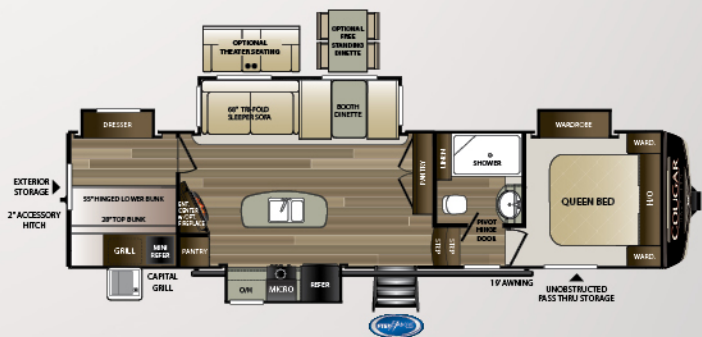
32DBH | Double bunkhouse w/ extra storage Weight: 9311 LBS. | Length: 35'5"
