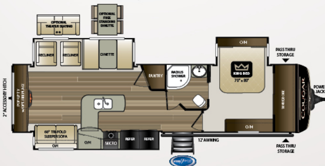
33SAB | Rear entertainment, double refrigerator Weight: 8847 LBS. | Length: 36' 11"
