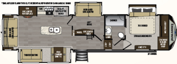
365MB/366MB | Center bonus room w/loft Weight: 12970 LBS. | Length: 39' 4"
