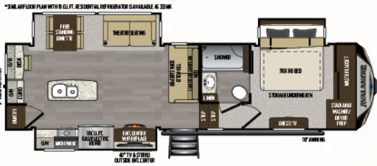
332MK/333MK | Mid-kitchen, triple-slide w/desk Weight: 11338 LBS. | Length: 34' 3"
