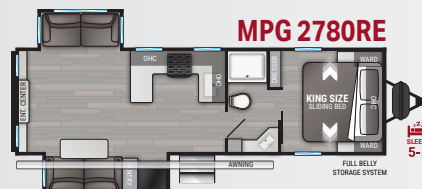
MPG 2780RE Length 31' 11" Height 11' 3" Dry 6482 lbs. Hitch 672 lbs.
