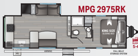
MPG 2975RK Length 33' 5" Height 11' 3" Dry 6634 lbs. Hitch 706 lbs.
