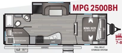
MPG 2500BH Length 29' 11" Height 11' 1" Dry 5828 lbs. Hitch 832 lbs.
