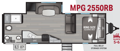
MPG 2550RB Length 30' 11" Height 11' 1" Dry 6062 lbs. Hitch 714 lbs.
