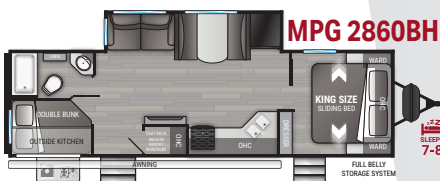
MPG 2860BH Length 32' 11" Height 11' 3" Dry 6724 lbs. Hitch 860 lbs.
