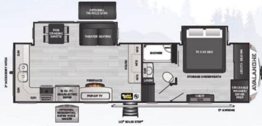
295RK | Rear kitchen, two slides, king bed WEIGHT 10701 LENGTH 33' 6"
