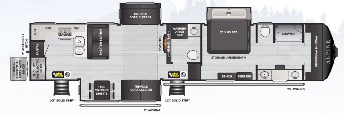
NEW! 3910RK | Rear kitchen, 1 1/2 bath, front bath master suite
