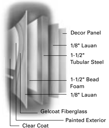
Fiberglass Sidewalls
