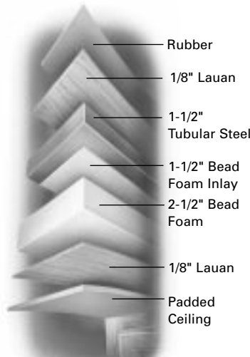
7-Layer Ceiling with Rubber Roof
