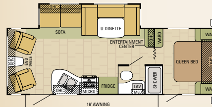
26RLS | LAUNCH ULTRA LITE
