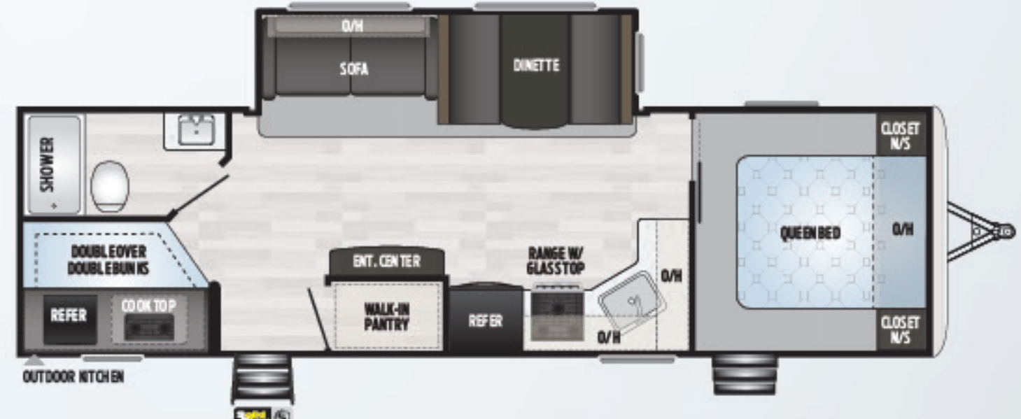
280BH | BUNKHOUSE, ENTERTAINMENT-FOCUSED, WALK-IN PANTRY & OUTSIDE KITCHEN Weight: 7167 LBS. | Length: 32' 11"
