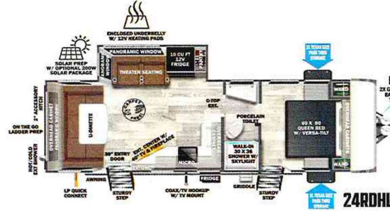
UVW = 6,228 lb Length = 29' 11"
