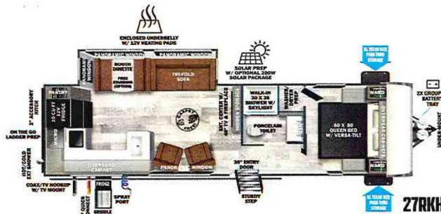
UVW = 6,758 lb Length = 34' 0"
