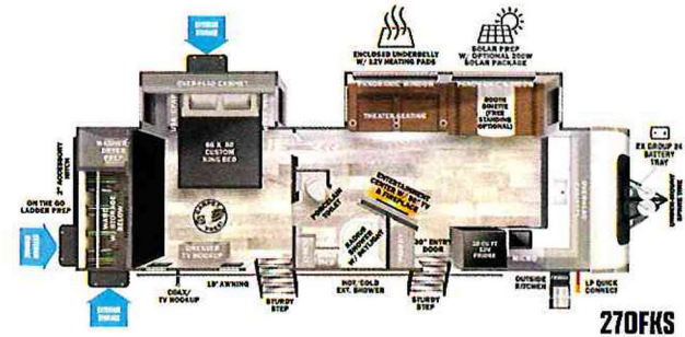
270FKS UVW = 8,243 lb Length = 33' 1"
