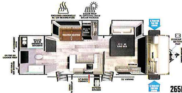
265BSRB UVW = 7,858 lb Length = 33' 2"
