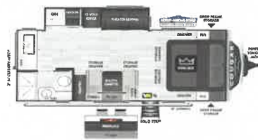
22MLS | WEIGHT 6086 | LENGTH 25' 9"
