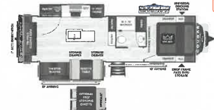
29RLP | WEIGHT 7875 | LENGTH 33' 7"
