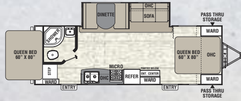
254 DSX ♦ Exterior Length 29' 7"
