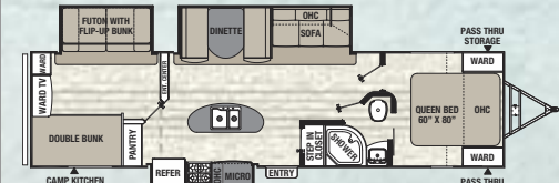
320 BHSLE ♦ Exterior Length 36' 11"
