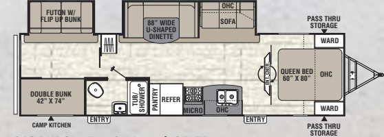
310 BHDS ♦ Exterior Length 35' 7"
