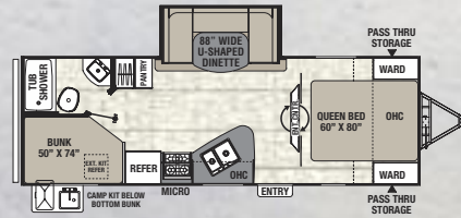
257 BHS ♦ Exterior Length 28' 7"
