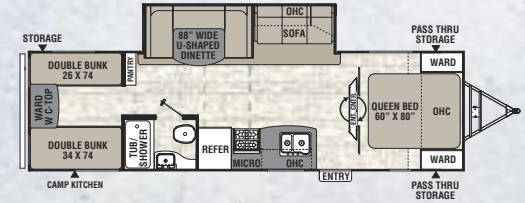
292 BHDS ♦ Exterior Length 33' 5"
