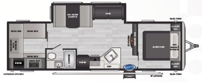
298BH | WEIGHT 6915 | LENGTH 32' 8"
