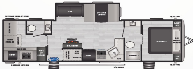
335BH | WEIGHT 8131 | LENGTH 37' 9"
