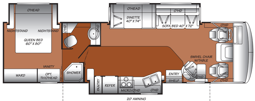
34F Triple Slide-Out Sleeping Accommodations: 4*
