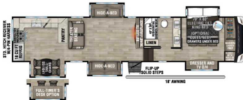
G391RKF UWW - 12,930 | Exterior Length - 42' 5" | Sleeps - 6
