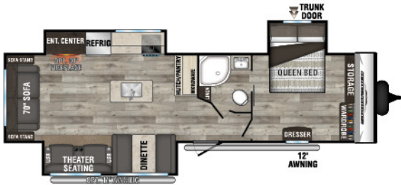
303QBSE UVW - 7,270 | Exterior Length - 34'7\"/>
