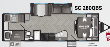
Length 31' 11" Dry 6,288 lbs. Hitch 816 lbs. Height 10' 11"
