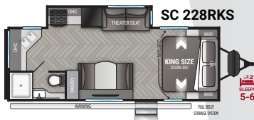
Length 26' 11" Dry 5,282 lbs. Hitch 654 lbs. Height 10' 11"
