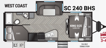
Length 27' 7" Dry 5,460 lbs. Hitch 660 lbs. Height 10' 11"
