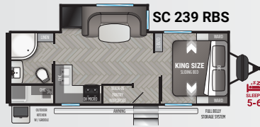
Length 27' 11" Dry 5,768 lbs. Hitch 670 lbs. Height 10' 11"
