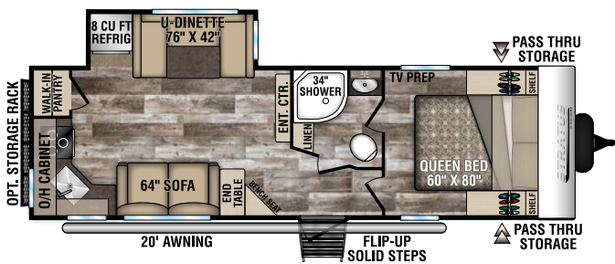
SR231VRB | 5,220 UVW | 26' 9" LENGTH | SLEEPS 4
