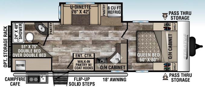
SR261VBH | 5,970 UVW | 30' 3" LENGTH | SLEEPS 8
