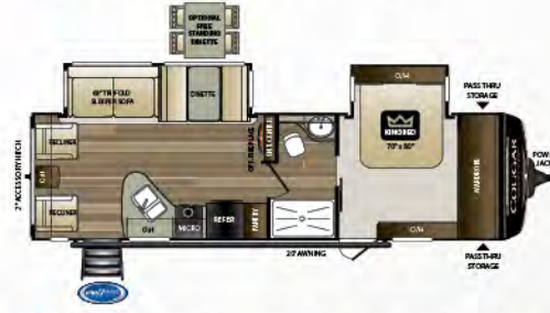
29RLD | Rear living room, bed slide w/ large front closet Weight: 7446 LBS. | Length: 33' 5"
