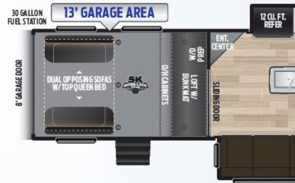
343 | TANDEM-AXLE, THREE SLIDES, 13' GARAGE
