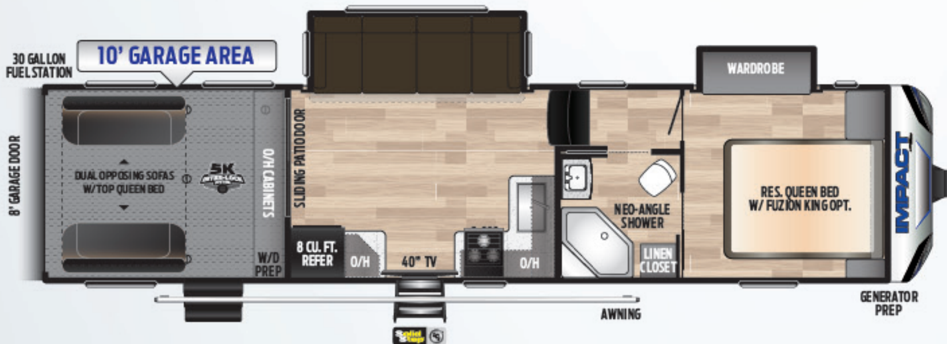
311 | TANDEM-AXLE, TWO SLIDES, 10' GARAGE | Weight: 11447 LBS. | Length: 35' 7"
