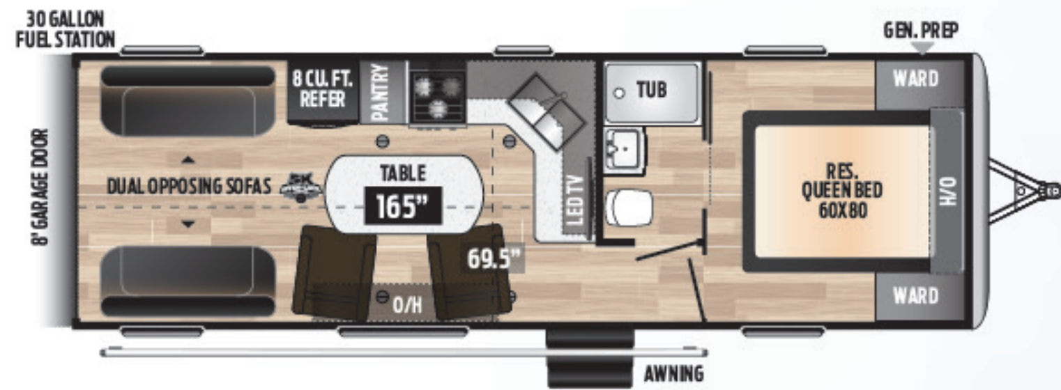
26V | LIGHTWEIGHT, OPEN CONCEPT, TANDEM-AXLE, 13' 9" GARAGE | Weight: 6645 LBS. | Length: 30' 6"
