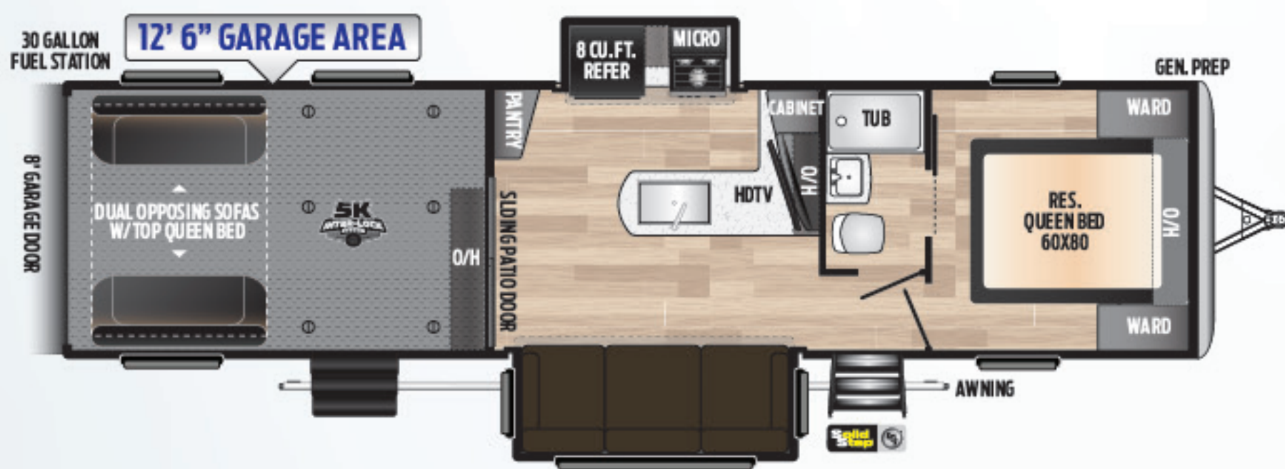
330 | TANDEM-AXLE, TWO SLIDES, 12' 6" GARAGE | Weight: 9454 LBS. | Length: 37' 6"
