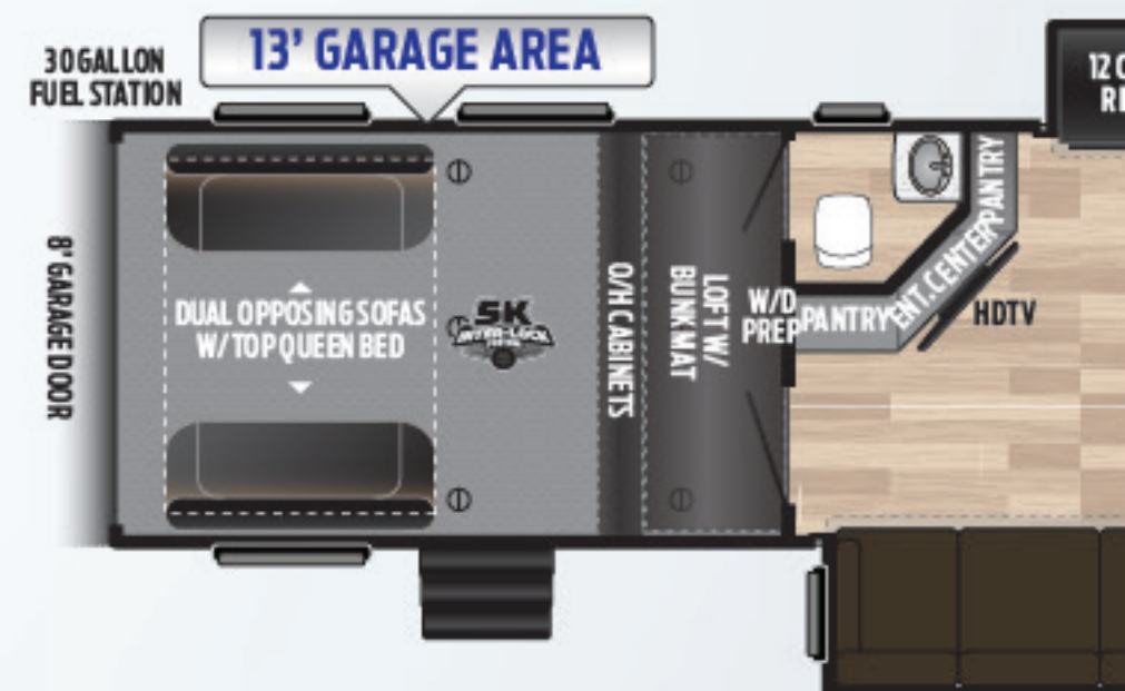
367 | TANDEM-AXLE, 1 1/2 BATH, 13' GARAGE
