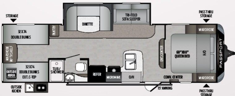
292BH | Quad bunkhouse w/ pack-n-play door Weight: 5743 LBS. | Length: 32' 4"
