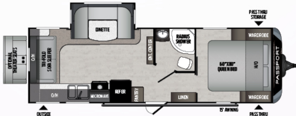
2521RLWE | Single-slide, ultimate couples coach GT SERIES | Weight: 5390 LBS. | Length: 32' 10"
