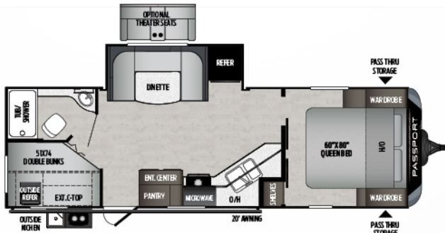
2600BH | Double over double bunkhouse, with outside kitchen Weight: 5580 LBS. | Length: 30' 8"
