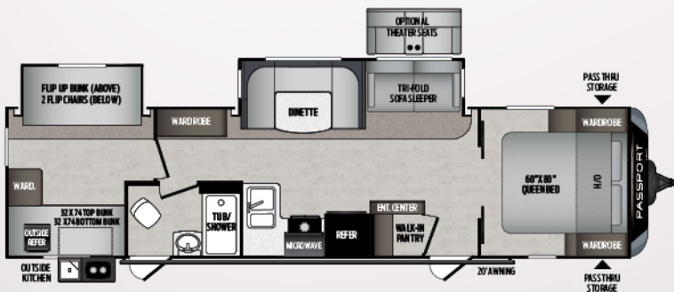
3221BH | Sleeps 8-10 w/outside kitchen Weight: 6785 LBS. | Length: 35' 5"
