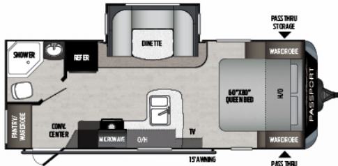
2210RBWE | Single-slide couple's coach GT SERIES | Weight: 4796 LBS. | Length: 26' 3"
