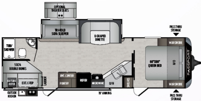
2820BH | Multi-purpose bunkhouse w/ outside kitchen Weight: 5875 | Length: 32' 11"
