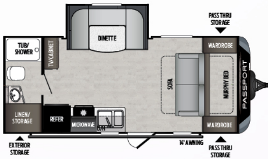
199ML | Single-slide couple's coach Weight: 4016 LBS. | Length: 22' 9"
