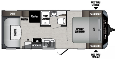
216RDWE | Couple's coach w/ oversized dinette SL SERIES | Weight: 4210 LBS. | Length: 24' 10"
