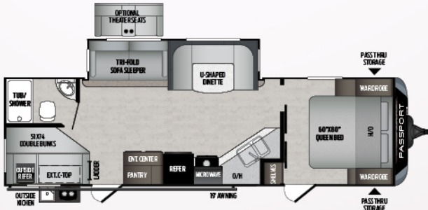
2820BHW | Multi-purpose bunkhouse w/ outside kitchen GT SERIES | Weight: 6070 | Length: 32' 11"
