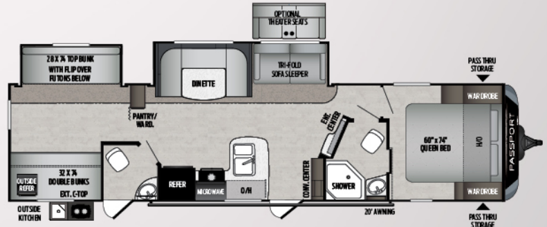
3351BH | Bath-N-Half bunkhouse Weight: 7020 LBS. | Length: 37' 7"
