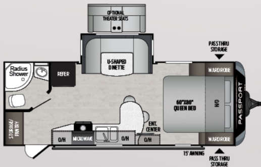
2210RB | Super slide w/ oversized bathroom Weight: 4760 LBS. | Length: 26' 3"
