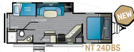
NT 24DBS LENGTH - 30' 10-1/2" | HEIGHT - 11' 4" | HITCH - 806 LBS. DRY - 6,316 LBS. | GVWR - 8,600 LBS. | SLEEP CAPACITY - 7-8
