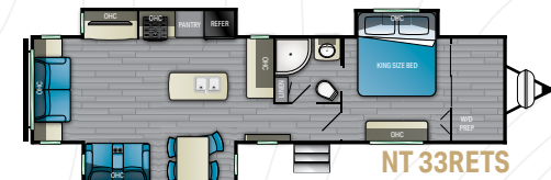
NT 33RETS LENGTH - 39' 8" | HEIGHT - 11' 8" | HITCH - 780 LBS. DRY - 8,840 LBS. | GVWR - 9,900 LBS. | SLEEP CAPACITY - 4
