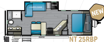
NT 25RBP LENGTH - 30' 10-1/2" | HEIGHT - 11' 4" | HITCH - 700 LBS. DRY - 6,278 LBS. | GVWR - 8,600 LBS. | SLEEP CAPACITY - 3-4
