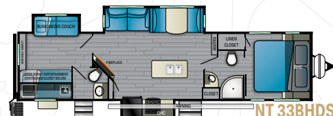
NT 33BHDS LENGTH - 37' 7-1/2" | HEIGHT - 11' 6" | HITCH - 992 LBS. DRY - 8,015 LBS. | GVWR - 9,600 LBS. | SLEEP CAPACITY - 9+
