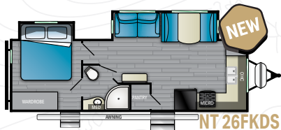
NT 26FKDS LENGTH - 29' 8 1/4" | HEIGHT - 11' 4" | HITCH - 972 LBS. DRY - 6,672 LBS. | GVWR - 9,772 LBS. | SLEEP CAPACITY - 5-6
