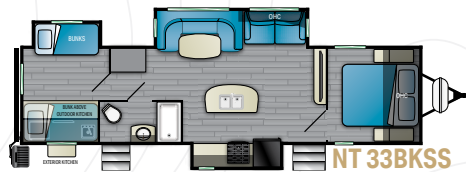
NT 33BKSS LENGTH - 36' 9-1/2" | HEIGHT - 11' 6" | HITCH - 774 LBS. DRY - 7,908 LBS. | GVWR - 9,600 LBS. | SLEEP CAPACITY - 9+
