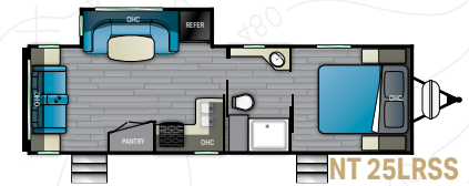
NT 25LRSS LENGTH - 31' 11" | HEIGHT - 11' 4" | HITCH - 688 LBS. DRY - 6,026 LBS. | GVWR - 7,400 LBS. | SLEEP CAPACITY - 3-4
