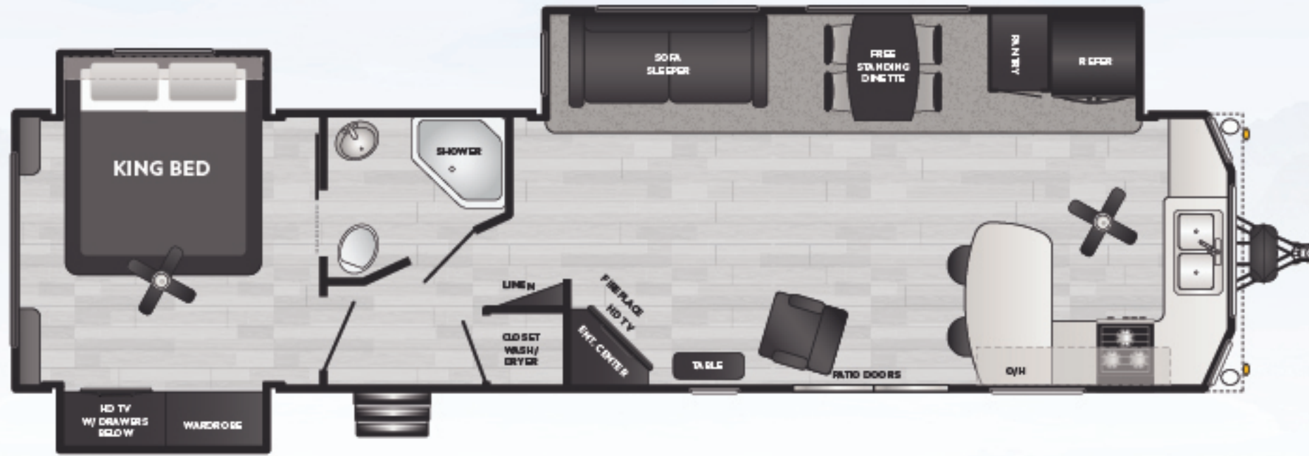
FKSS | Three slides w/king bed, front kitchen, patio door
