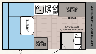
JAY SERIES SPORT HARDWALL | 12BSB Ext. Length: 18' 8" Travel Ht.: 58" Unloaded Wt. (lbs.): 2,135 Sleeps: 2
