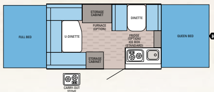
JAY SERIES SPORT | 12UD Ext. Length: 15' 6" Travel Ht.: 57" Unloaded Wt. (lbs.): 1,570 Sleeps: 6-7
