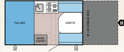
JAY SERIES SPORT HARDWALL | 12HFD Ext. Length: 22' 4" Travel Ht.: 71" Unloaded Wt. (lbs.): 2,385 Sleeps: 3-4
