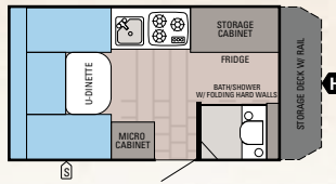
JAY SERIES SPORT HARDWALL | 12BMD Ext. Length: 18' 8" Travel Ht.: 62" Unloaded Wt. (lbs.): 2,005 Sleeps: 2
