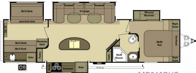
MR310BHS Ext. Length: 37'3" Ext. Height: 140" UVW (lbs.): 9310 Sleeps: 8
