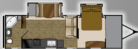
Length: 32' 6" Dry: 6,695 NT 26BRSS Height: 11' 4" Hitch: 678 GVWR: 8,600
