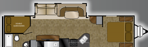
Length: 35' 11" Dry: 6,399 NT 31BHDD Height: 11' 4" Hitch: 652 GVWR: 8,600
