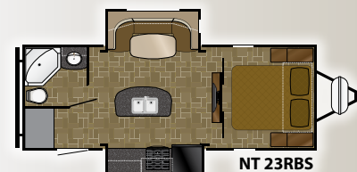
Length: 26' 11" Dry: 5,310 NT 23RBS Height: 11' 2" Hitch: 625 GVWR: 6,900
