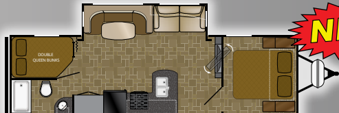
Length: 33' 6" Dry: 6,432 NT 28DBSS Height: 11' 4" Hitch: 644 GVWR: 8,600
