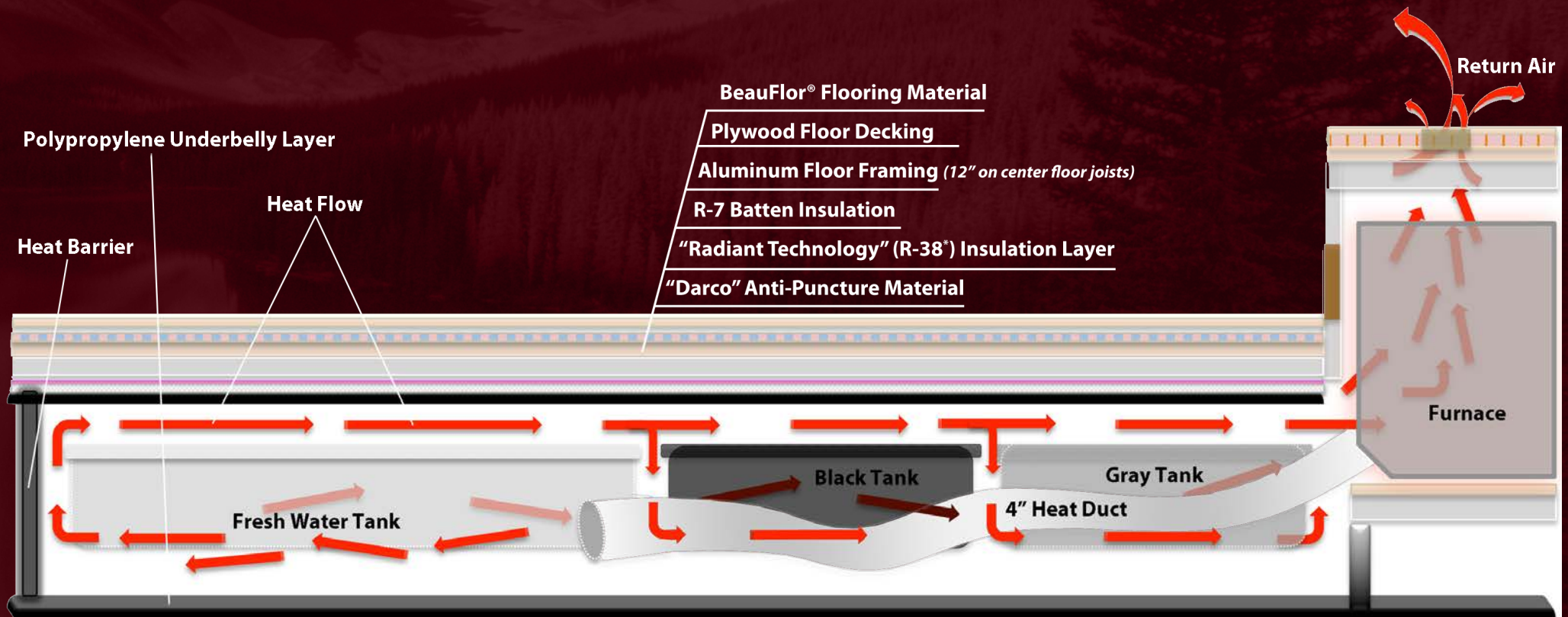
*Mesa Ridge Fifth Wheel Diagram Shown
