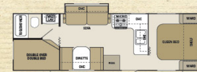
Launch Ultra Lite 26BHS
