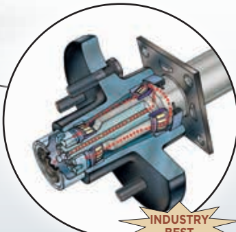
AL-KO® Ultralube axle bearing. Easier maintenance for improved safety
