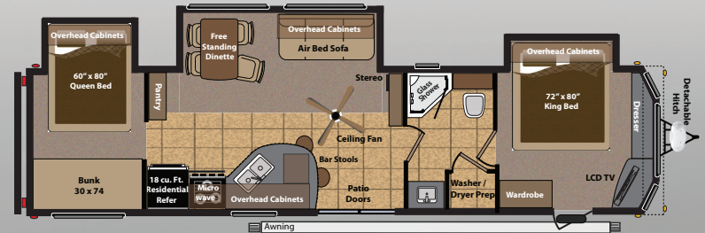
402BH LENGTH: 40' 11" WEIGHT: 11,713
