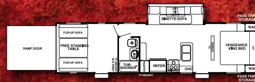
T300V - 10ft garage
