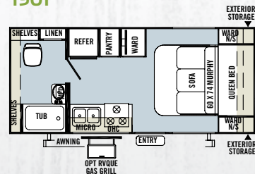
Murphy Bed Shown in the Down Position
