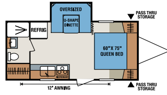
S202SRB • Twin Beds Option – see below
