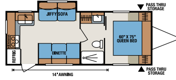
S241RKS • Twin Beds Option – see below
