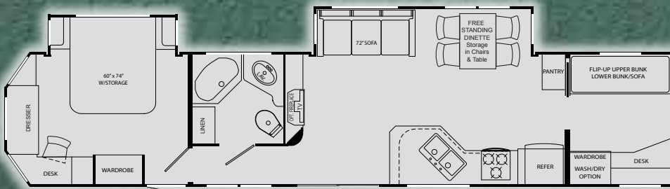
Length: 44'-8" • Height: 12'-9" • GVWR: 14,000 lb. 41RBQB
