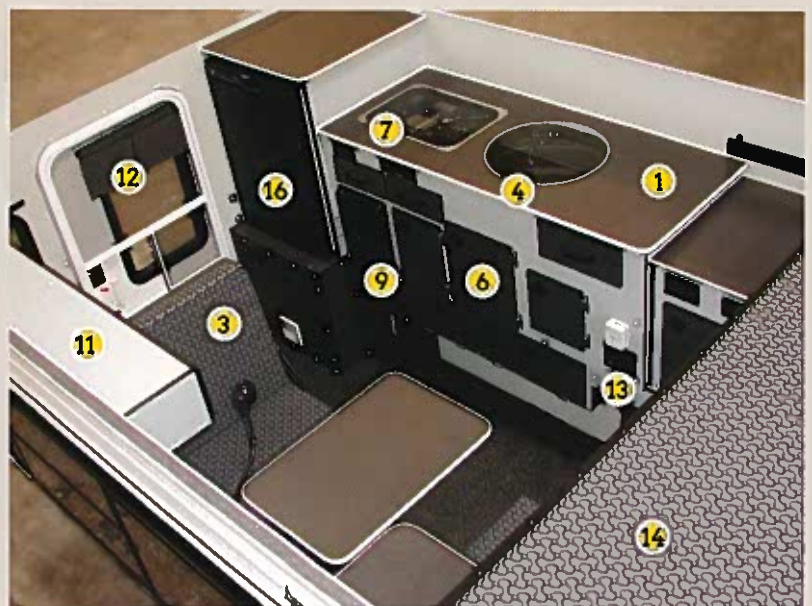
Side Dinette Seating | Silver Spur Interior
