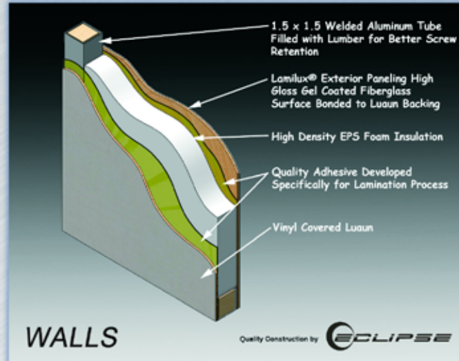
Fiberglass-Laminated, Aluminum-Framed
